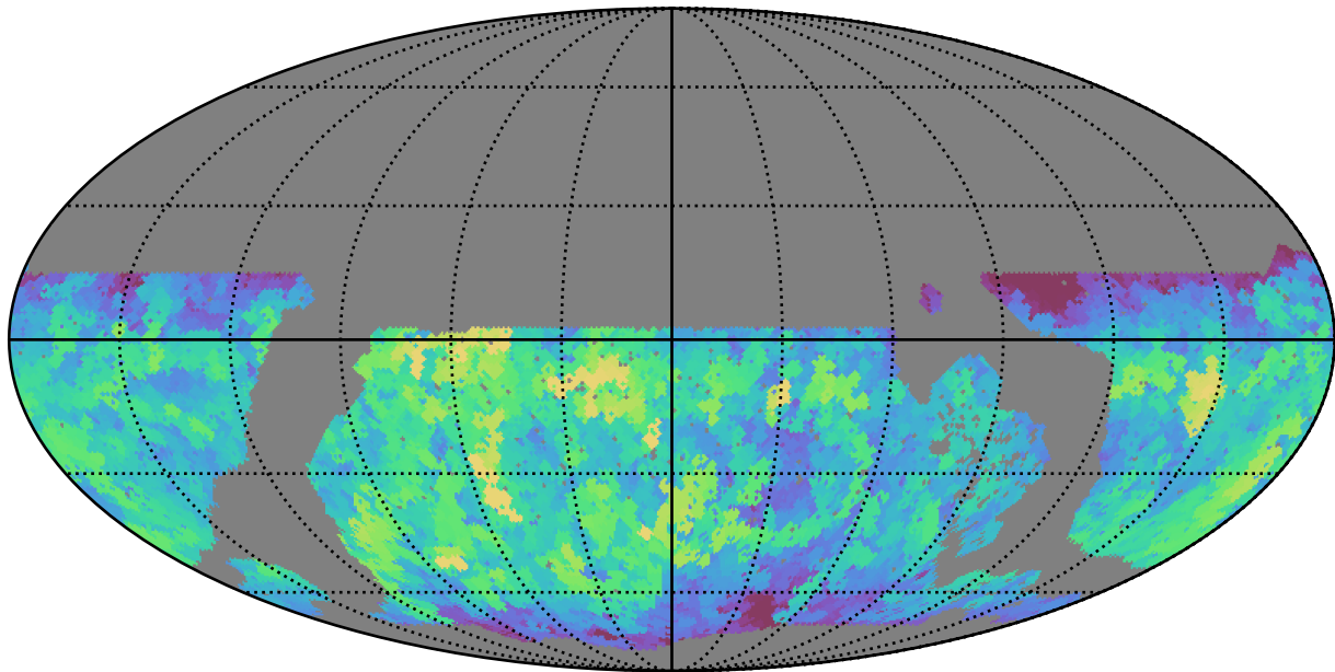
noroll_mjdp120_v3.4_10yrs WFD g band: Max saturation_mag
