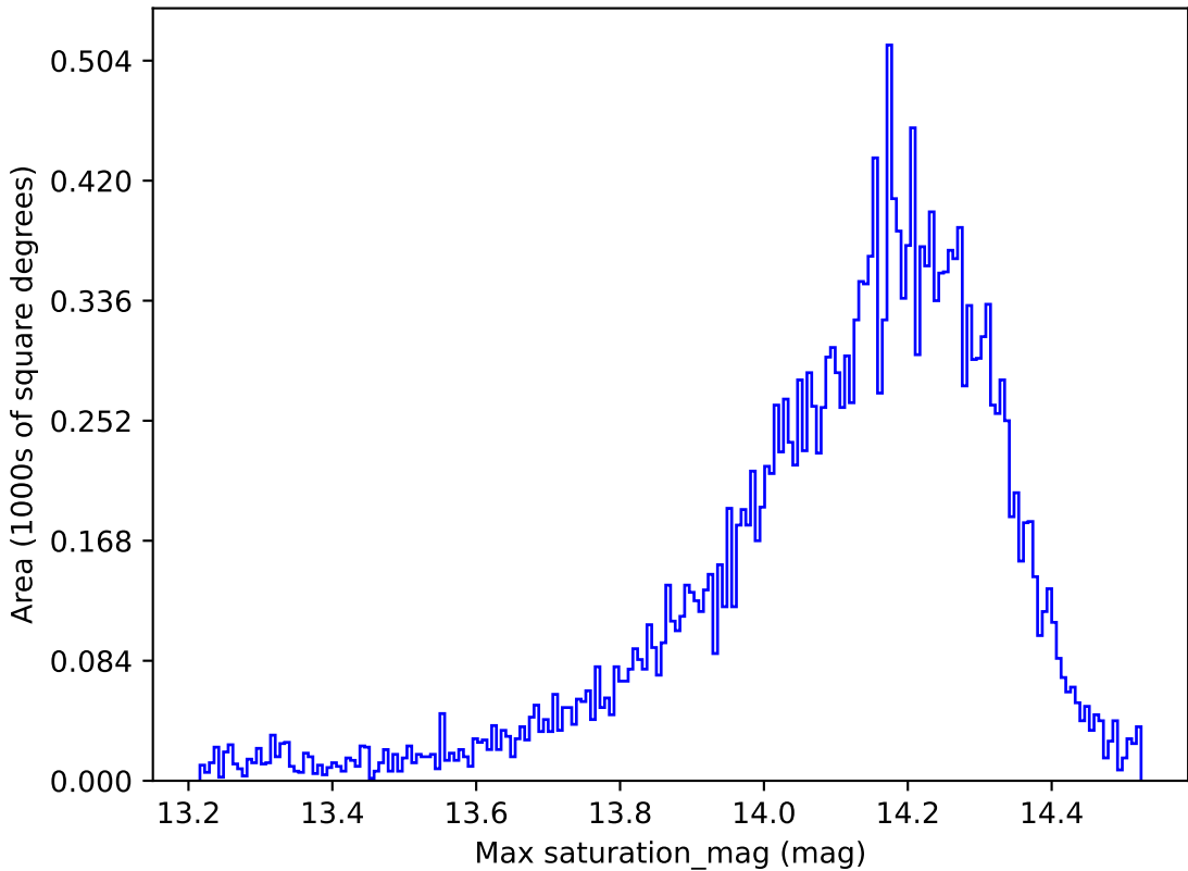
noroll_mjdp120_v3.4_10yrs All sky y band: Max saturation_mag
