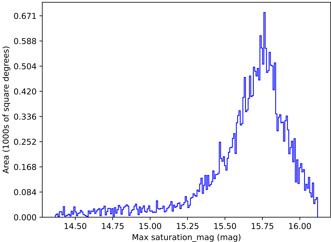
noroll_mjdp120_v3.4_10yrs All sky r band: Max saturation_mag
