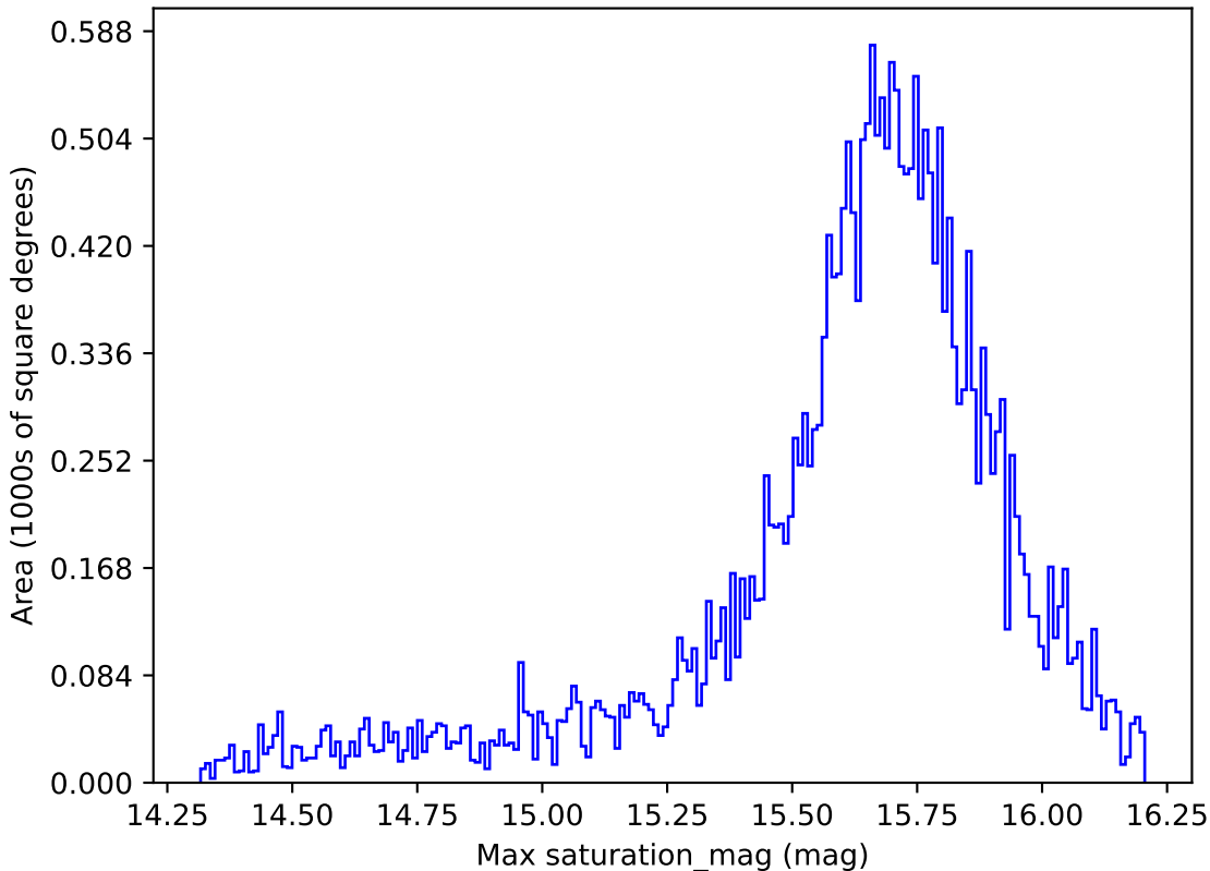
noroll_mjdp120_v3.4_10yrs All sky g band: Max saturation_mag
