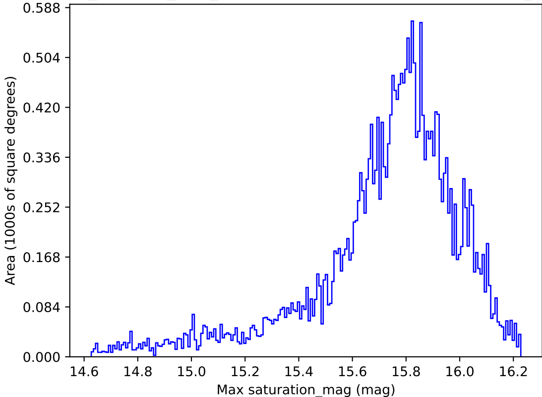
noroll_mjdp120_v3.4_10yrs All sky all bands: Max saturation_mag
