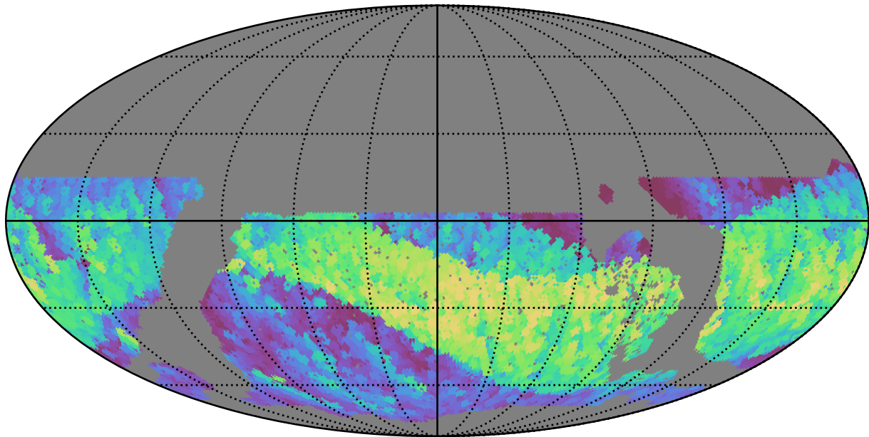
noroll_mjdp120_v3.4_10yrs WFD z band: Max normairmass
