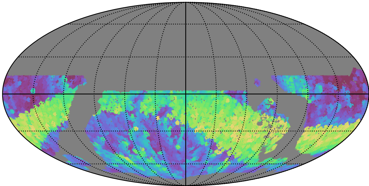
noroll_mjdp120_v3.4_10yrs WFD r band: Max normairmass
