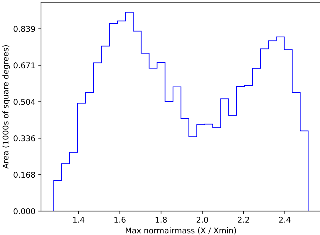
noroll_mjdp120_v3.4_10yrs WFD r band: Max normairmass
