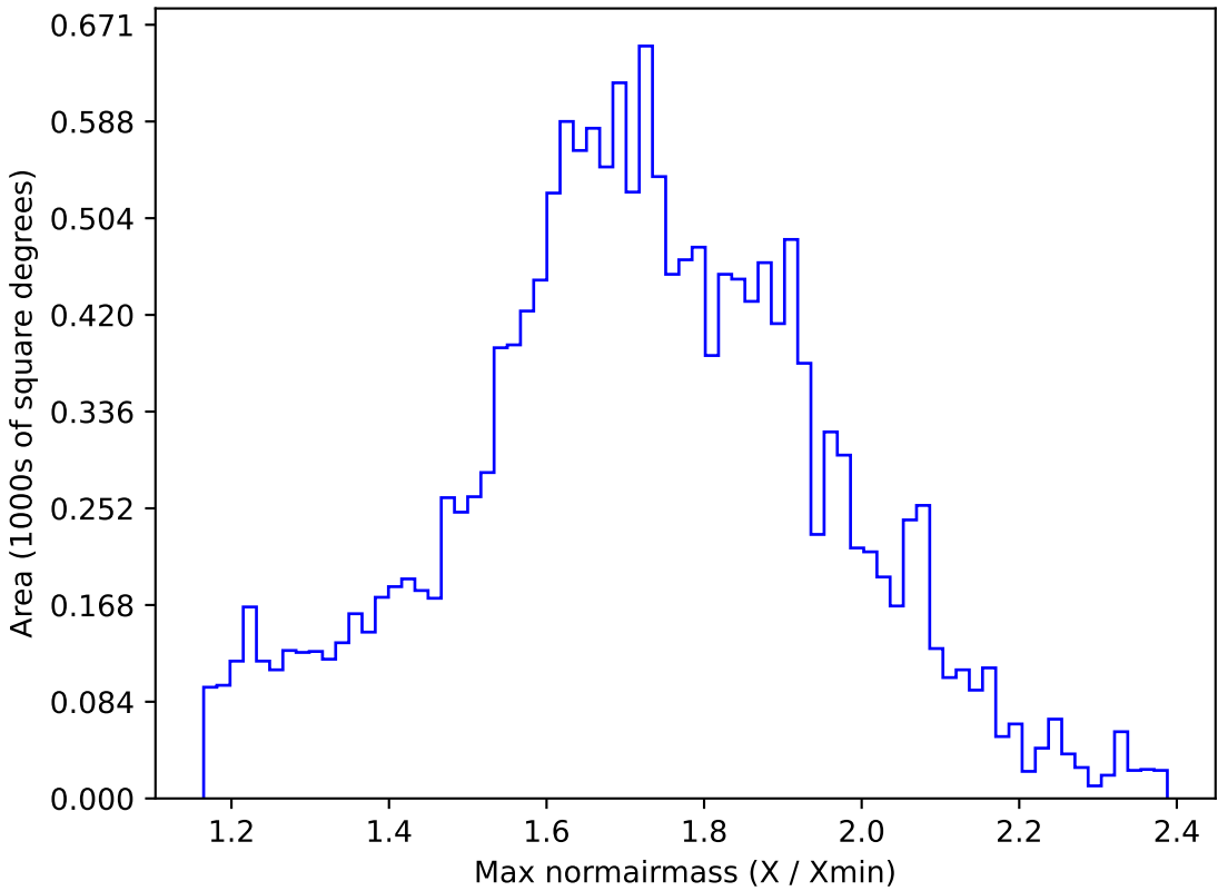
noroll_mjdp120_v3.4_10yrs WFD g band: Max normairmass
