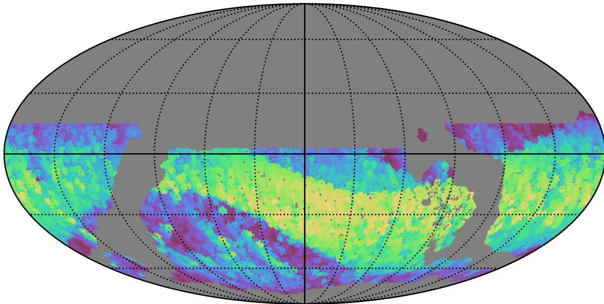
noroll_mjdp120_v3.4_10yrs WFD all bands: Max normairmass
