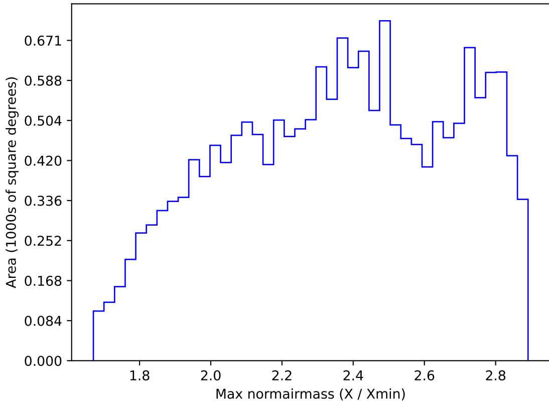
noroll_mjdp120_v3.4_10yrs WFD all bands: Max normairmass
