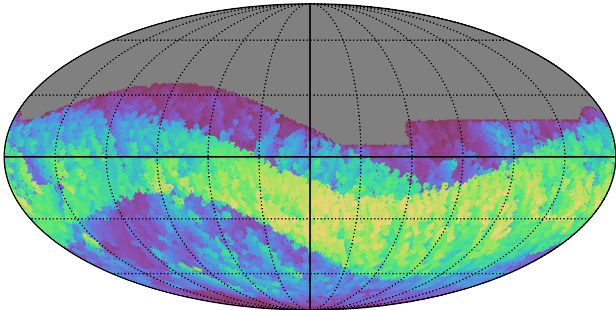
noroll_mjdp120_v3.4_10yrs All sky z band: Max normairmass
