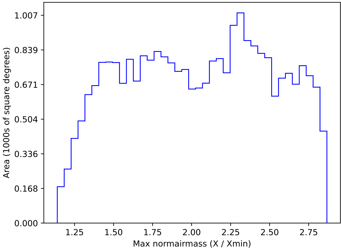
noroll_mjdp120_v3.4_10yrs All sky z band: Max normairmass
