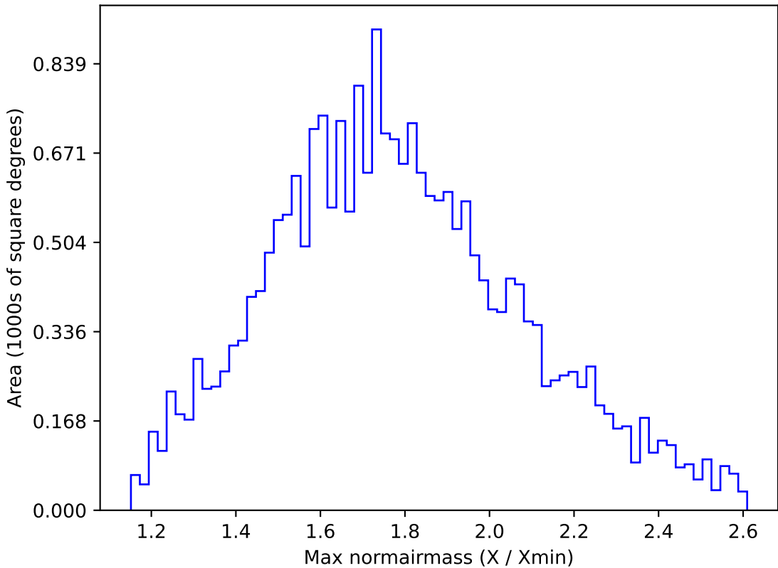
noroll_mjdp120_v3.4_10yrs All sky y band: Max normairmass
