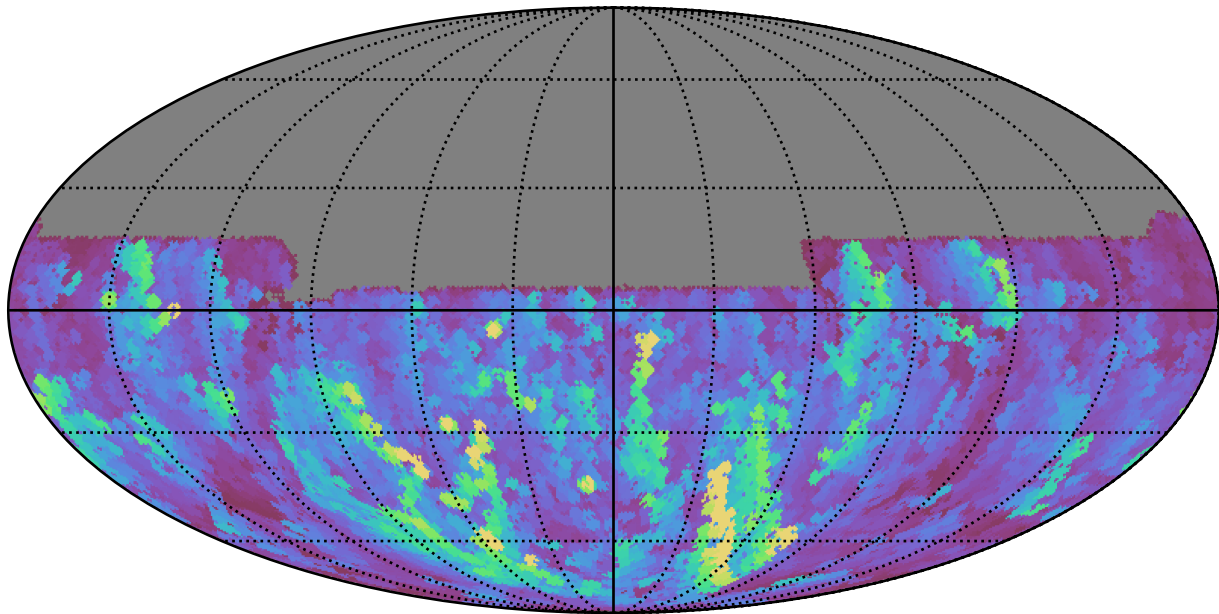
noroll_mjdp120_v3.4_10yrs All sky u band: Max normairmass
