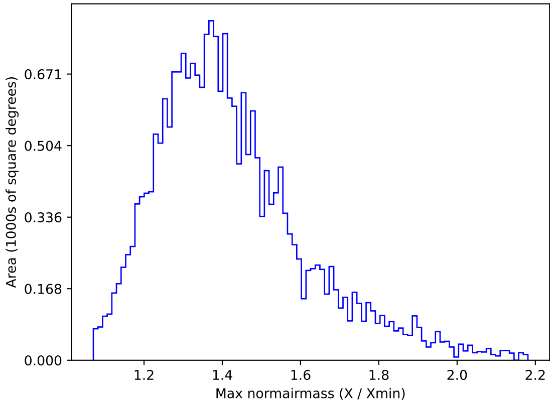
noroll_mjdp120_v3.4_10yrs All sky u band: Max normairmass
