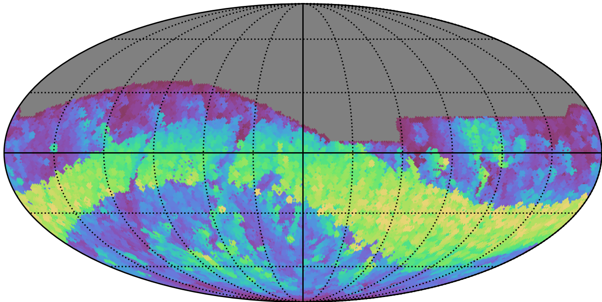
noroll_mjdp120_v3.4_10yrs All sky r band: Max normairmass
