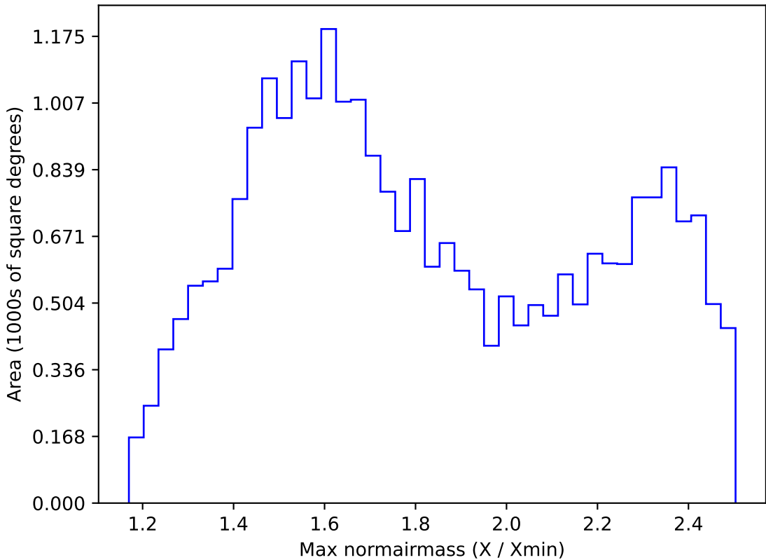
noroll_mjdp120_v3.4_10yrs All sky r band: Max normairmass
