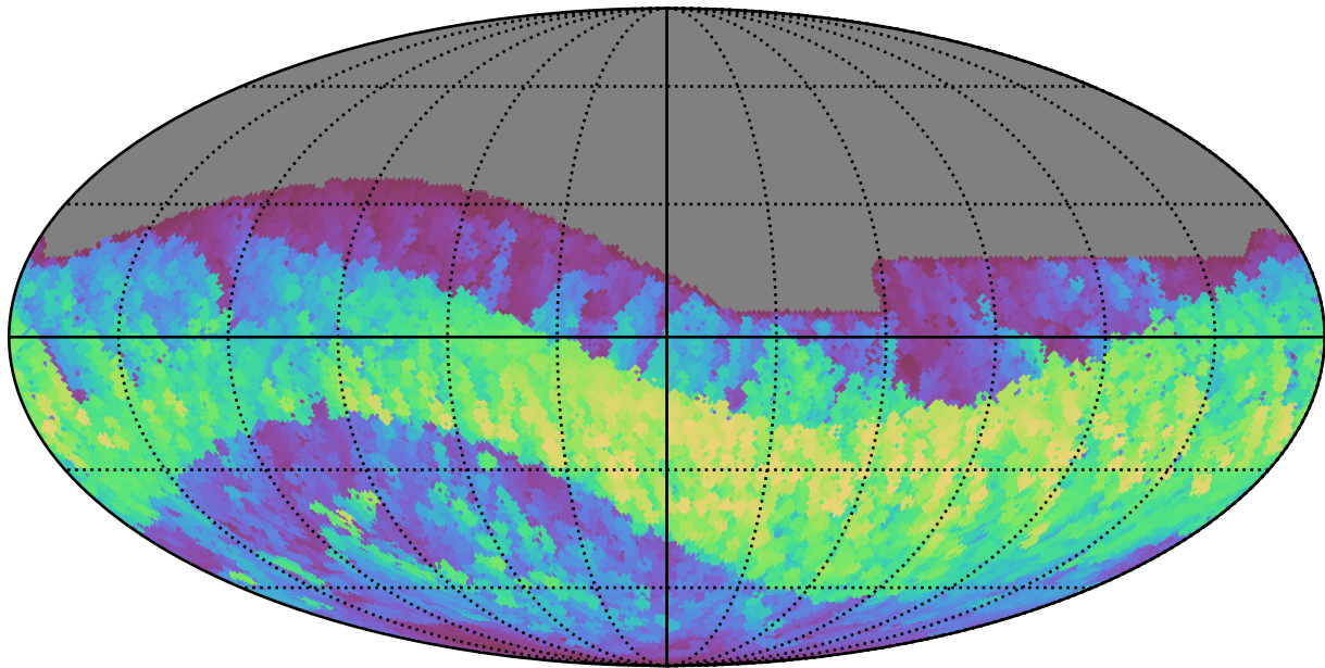
noroll_mjdp120_v3.4_10yrs All sky i band: Max normairmass
