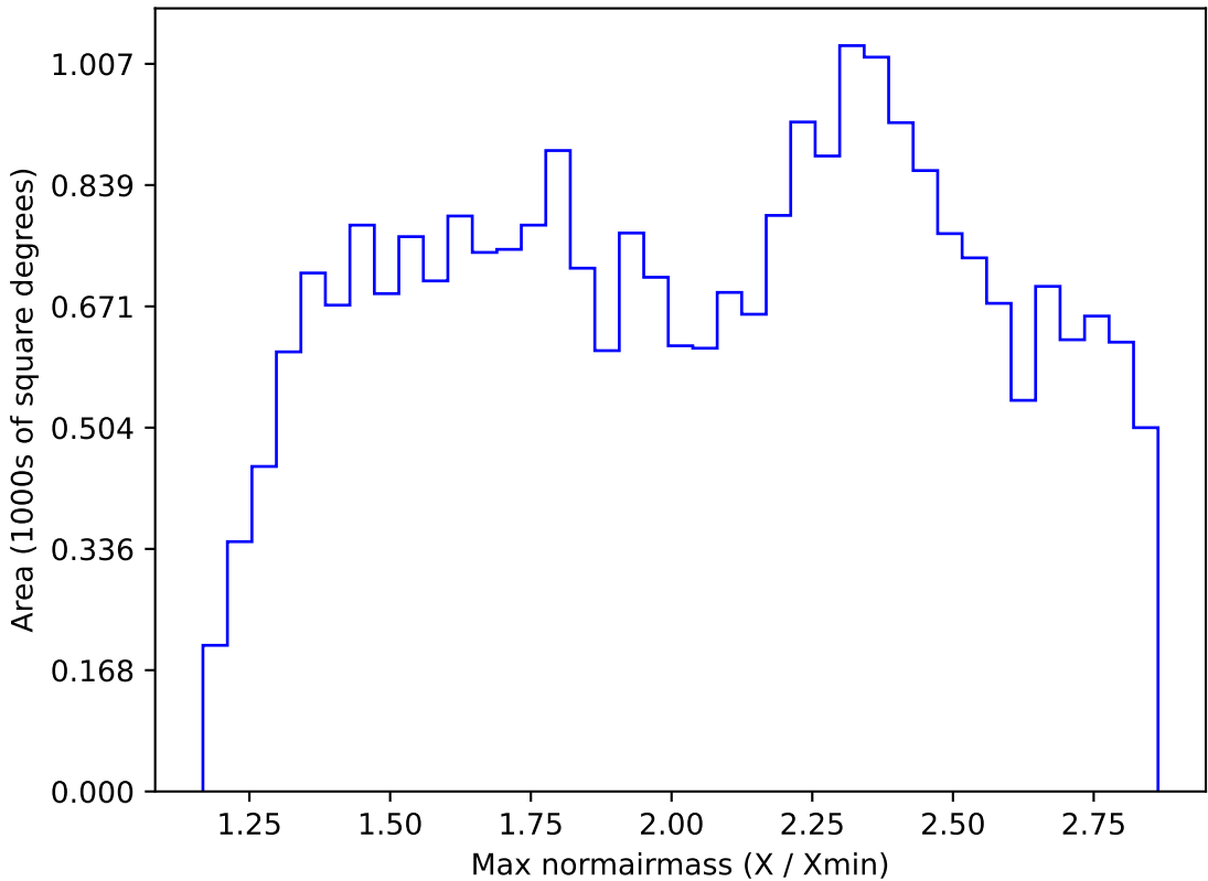
noroll_mjdp120_v3.4_10yrs All sky i band: Max normairmass
