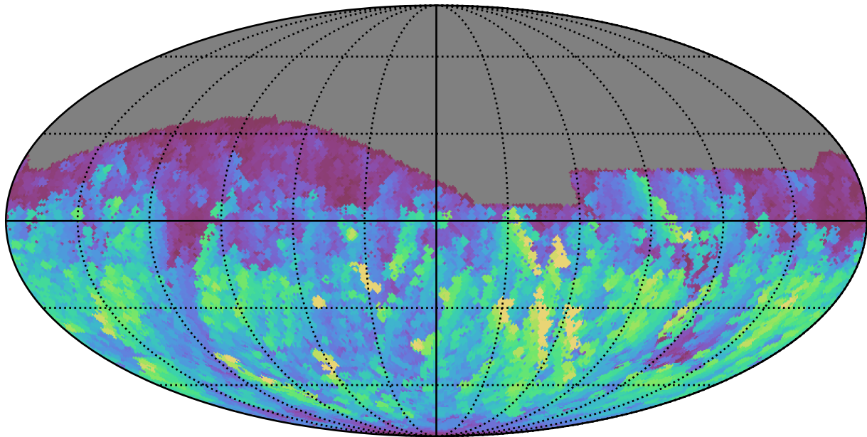
noroll_mjdp120_v3.4_10yrs All sky g band: Max normairmass
