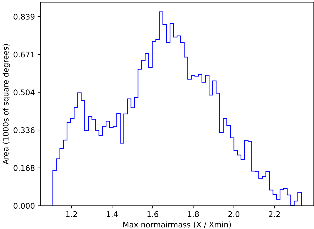
noroll_mjdp120_v3.4_10yrs All sky g band: Max normairmass
