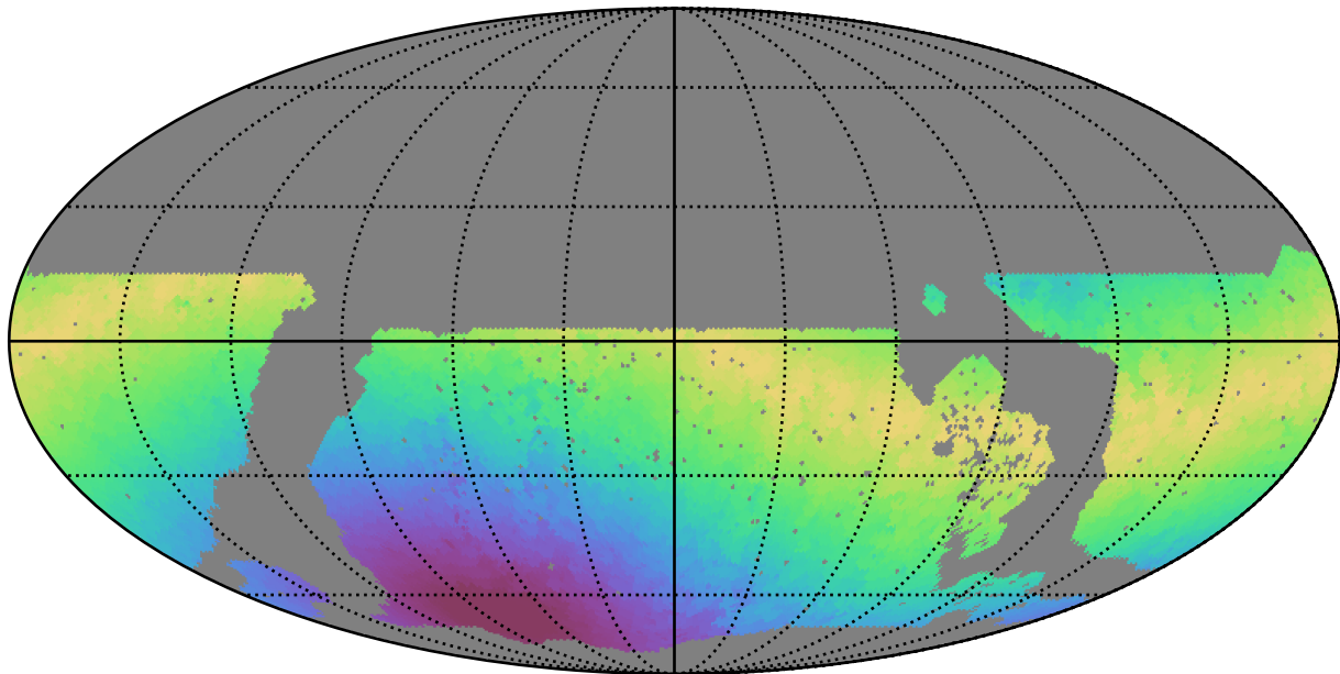
noroll_mjdp120_v3.4_10yrs WFD z band: Max moonDistance
