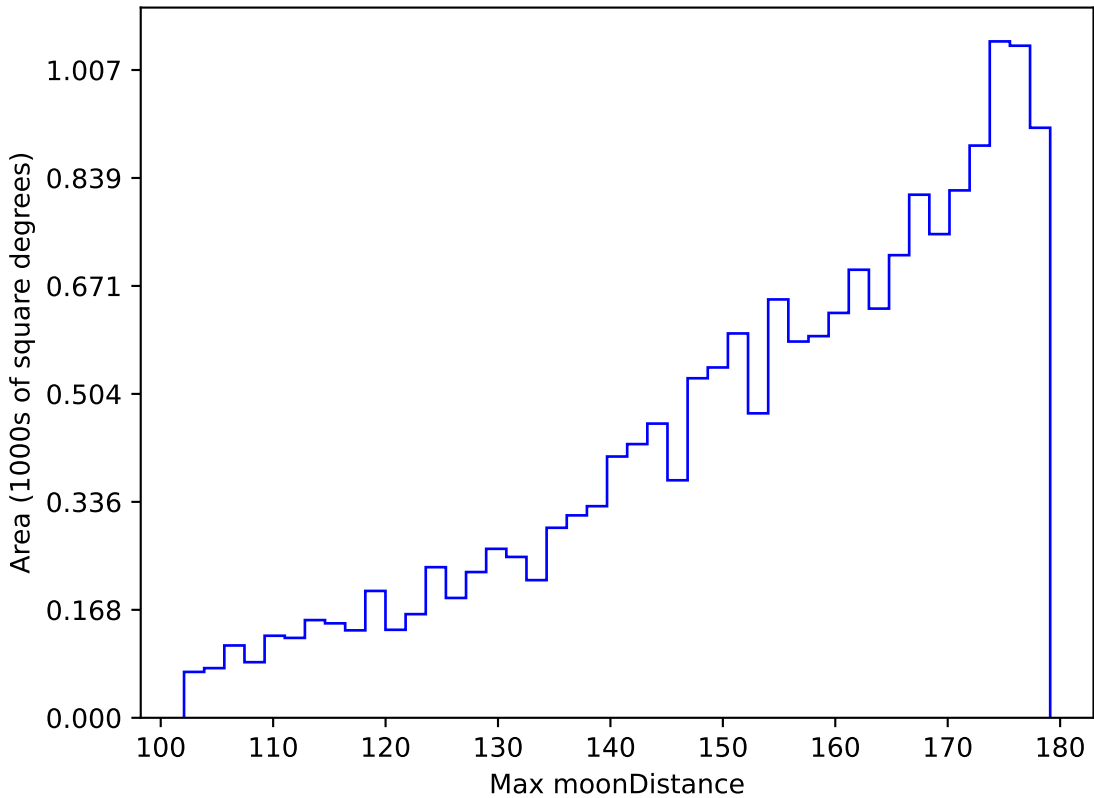
noroll_mjdp120_v3.4_10yrs WFD u band: Max moonDistance
