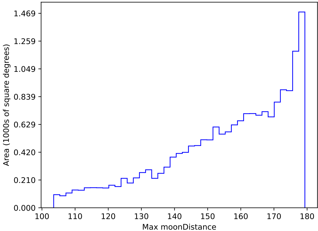
noroll_mjdp120_v3.4_10yrs WFD r band: Max moonDistance
