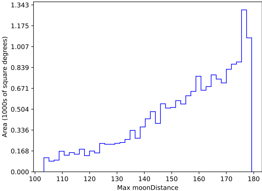
noroll_mjdp120_v3.4_10yrs WFD i band: Max moonDistance
