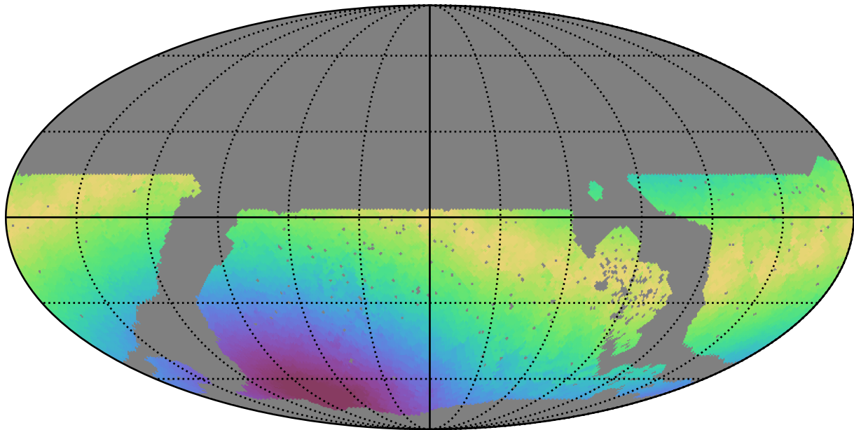
noroll_mjdp120_v3.4_10yrs WFD g band: Max moonDistance
