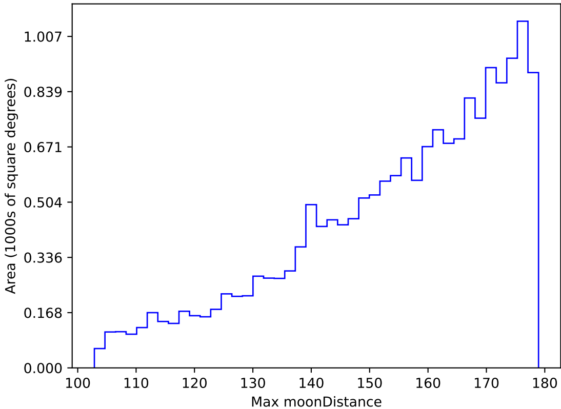
noroll_mjdp120_v3.4_10yrs WFD g band: Max moonDistance
