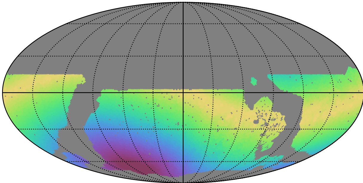
noroll_mjdp120_v3.4_10yrs WFD all bands: Max moonDistance
