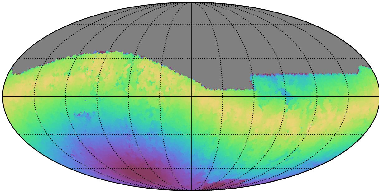
noroll_mjdp120_v3.4_10yrs All sky z band: Max moonDistance
