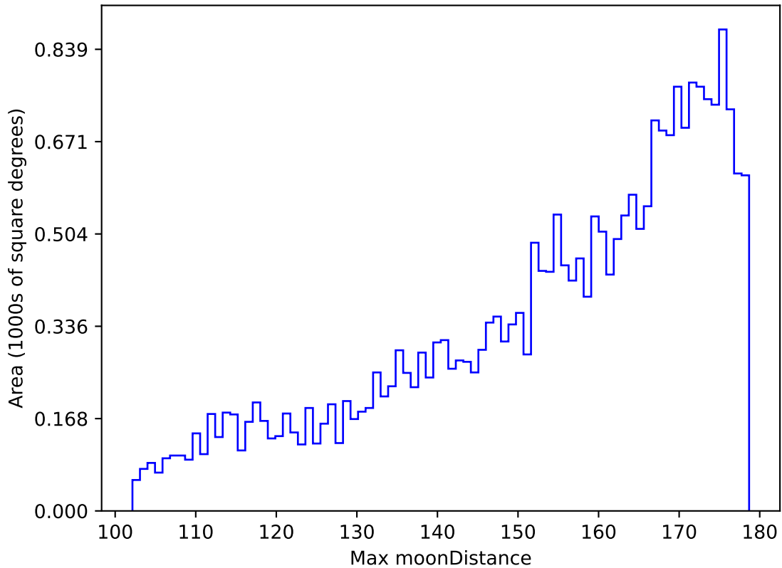
noroll_mjdp120_v3.4_10yrs All sky z band: Max moonDistance
