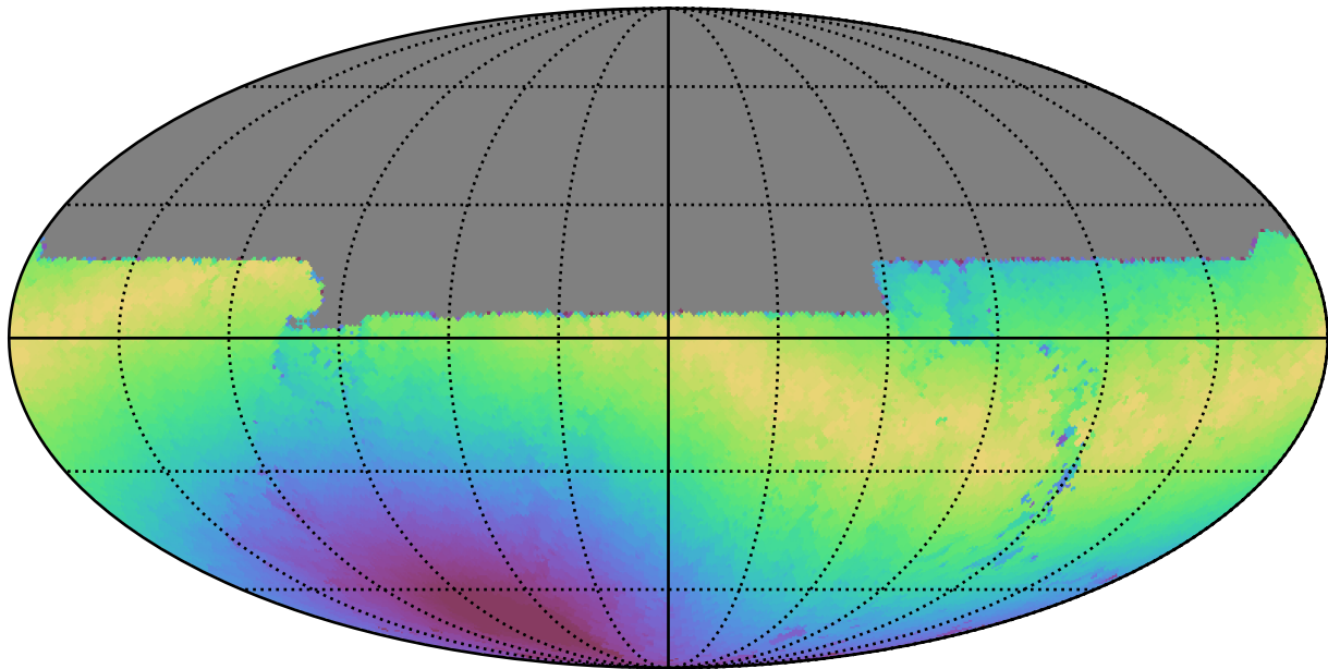
noroll_mjdp120_v3.4_10yrs All sky u band: Max moonDistance
