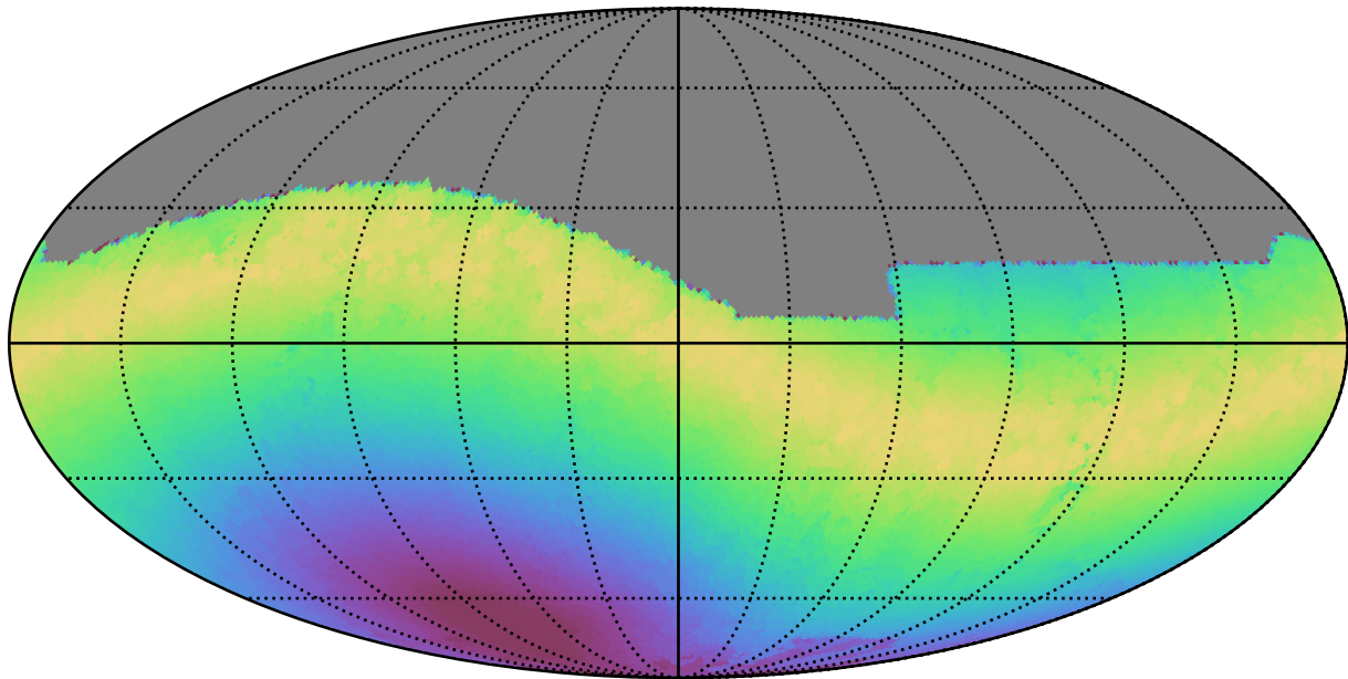
noroll_mjdp120_v3.4_10yrs All sky r band: Max moonDistance
