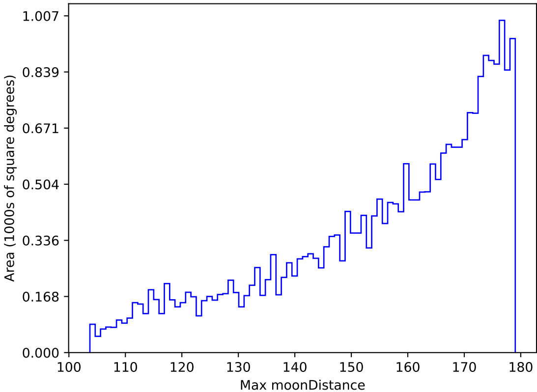
noroll_mjdp120_v3.4_10yrs All sky i band: Max moonDistance
