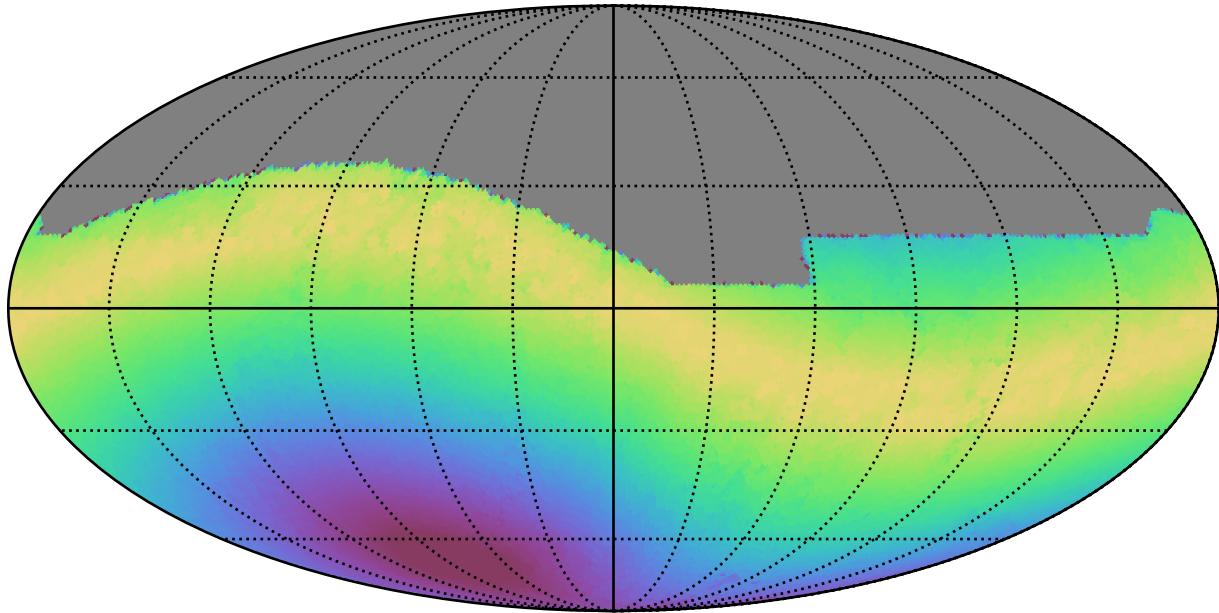
noroll_mjdp120_v3.4_10yrs All sky all bands: Max moonDistance
