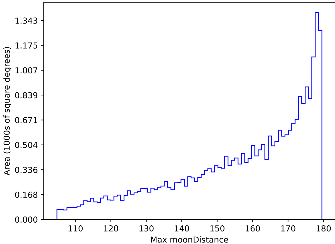
noroll_mjdp120_v3.4_10yrs All sky all bands: Max moonDistance
