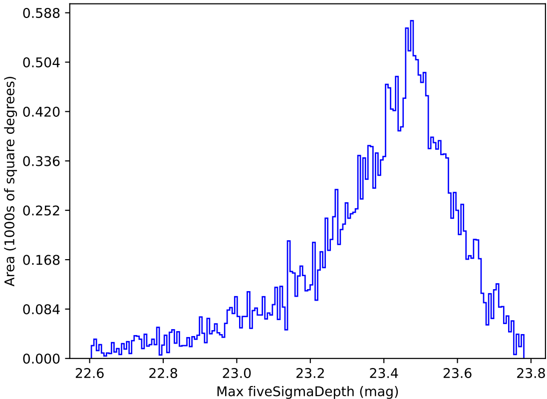
noroll_mjdp120_v3.4_10yrs Yr 1 z band: Max fiveSigmaDepth
