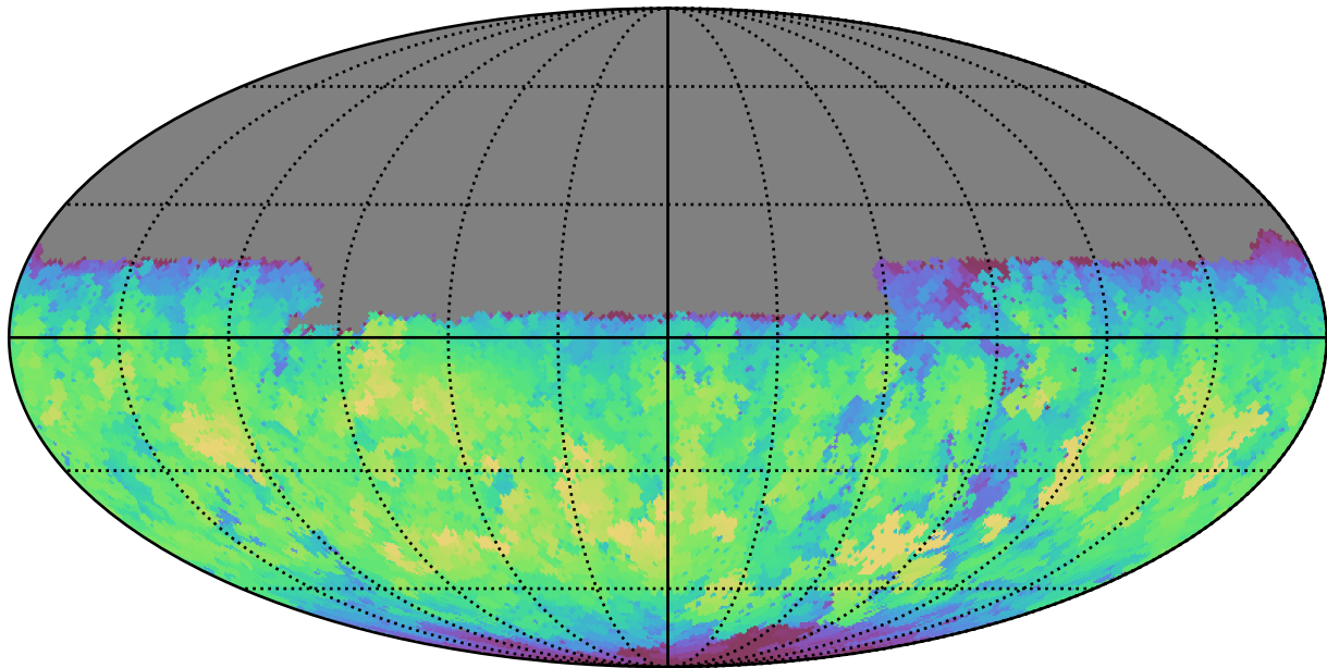
noroll_mjdp120_v3.4_10yrs Yr 1 y band: Max fiveSigmaDepth
