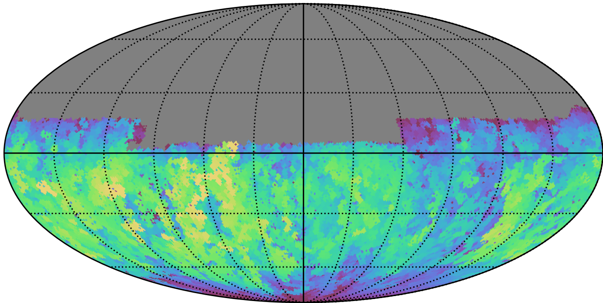
noroll_mjdp120_v3.4_10yrs Yr 1 u band: Max fiveSigmaDepth
