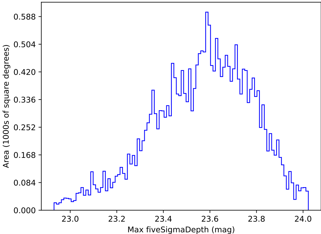
noroll_mjdp120_v3.4_10yrs Yr 1 u band: Max fiveSigmaDepth
