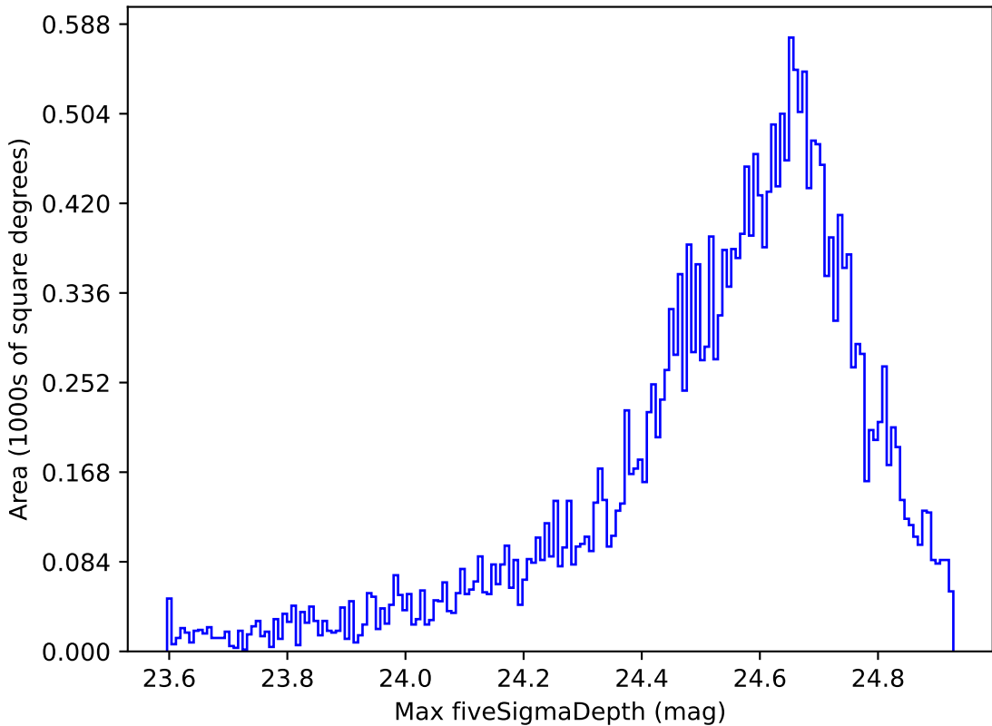
noroll_mjdp120_v3.4_10yrs Yr 1 r band: Max fiveSigmaDepth
