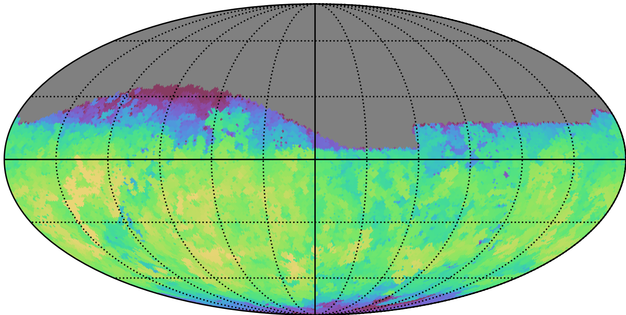
noroll_mjdp120_v3.4_10yrs Yr 1 i band: Max fiveSigmaDepth
