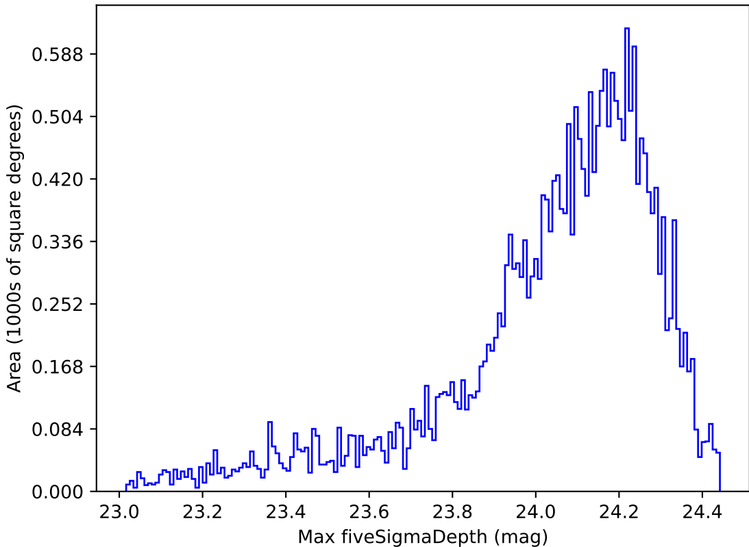
noroll_mjdp120_v3.4_10yrs Yr 1 i band: Max fiveSigmaDepth
