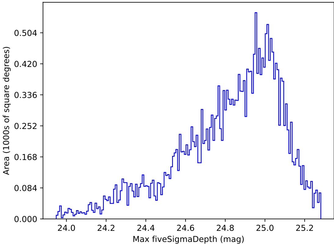
noroll_mjdp120_v3.4_10yrs Yr 1 g band: Max fiveSigmaDepth
