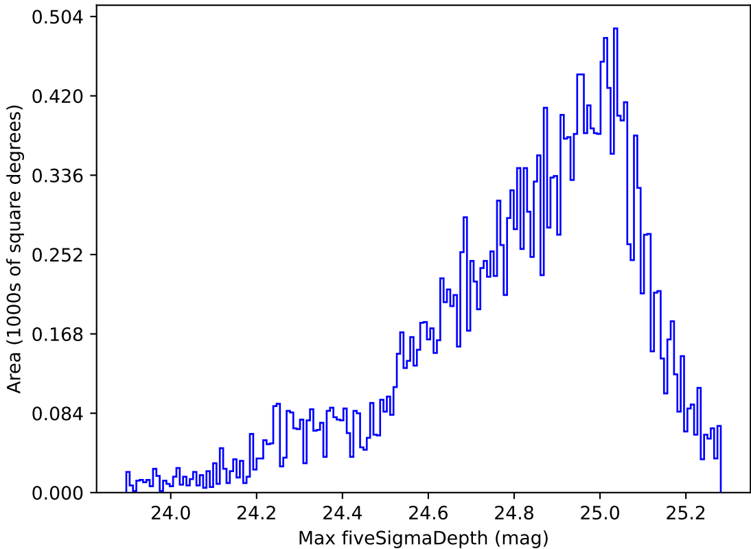
noroll_mjdp120_v3.4_10yrs Yr 1 all bands: Max fiveSigmaDepth
