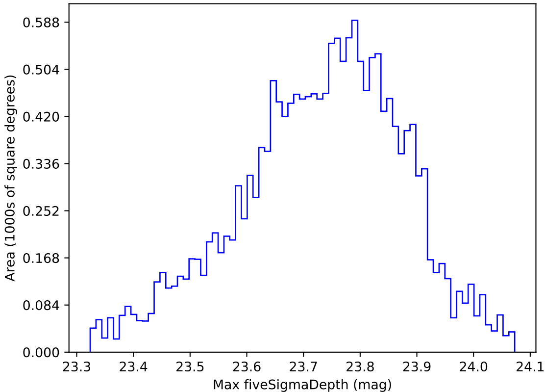
noroll_mjdp120_v3.4_10yrs WFD u band: Max fiveSigmaDepth
