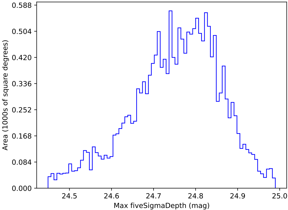
noroll_mjdp120_v3.4_10yrs WFD r band: Max fiveSigmaDepth
