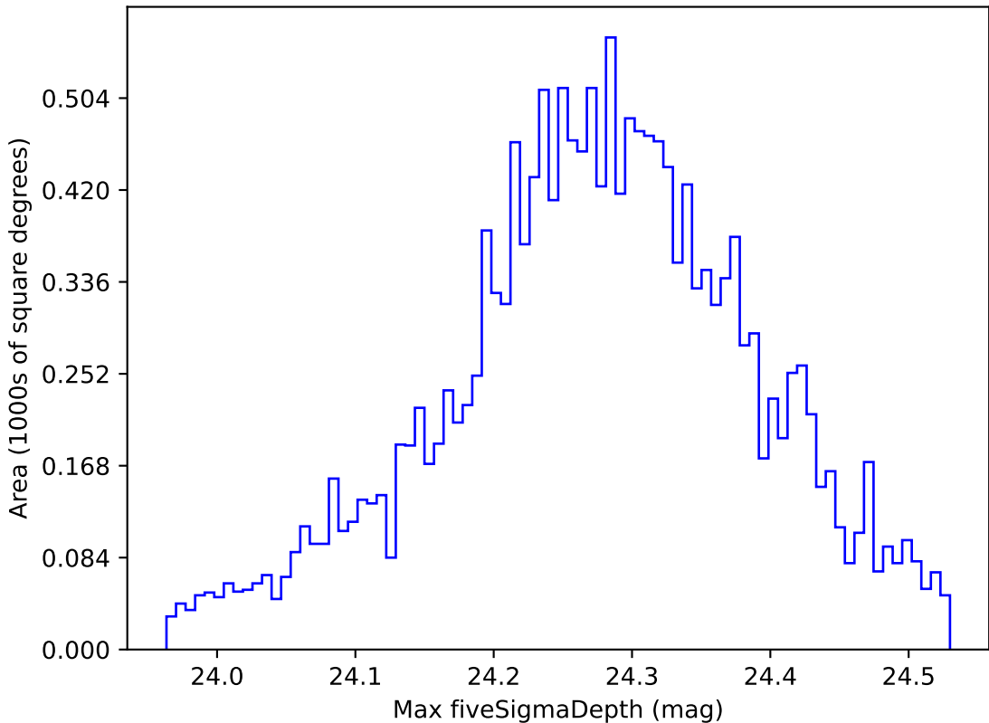
noroll_mjdp120_v3.4_10yrs WFD i band: Max fiveSigmaDepth
