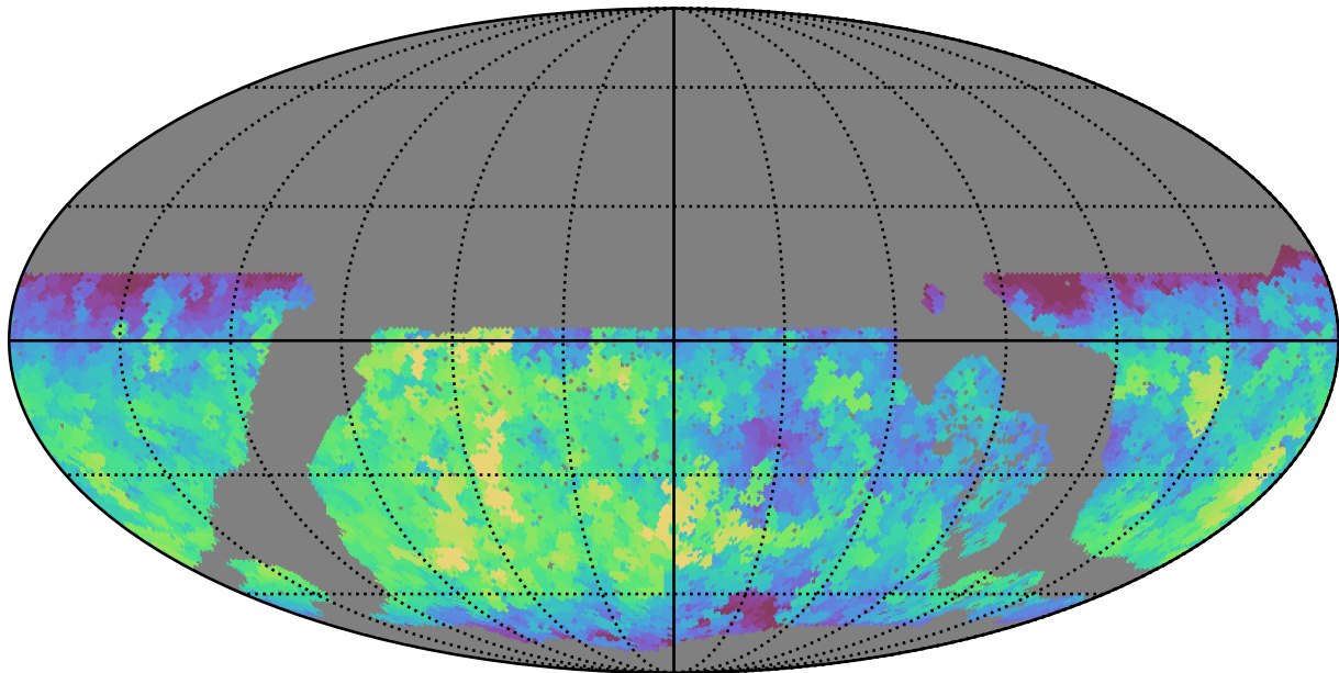
noroll_mjdp120_v3.4_10yrs WFD g band: Max fiveSigmaDepth
