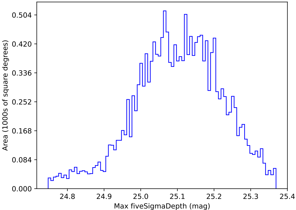
noroll_mjdp120_v3.4_10yrs WFD g band: Max fiveSigmaDepth
